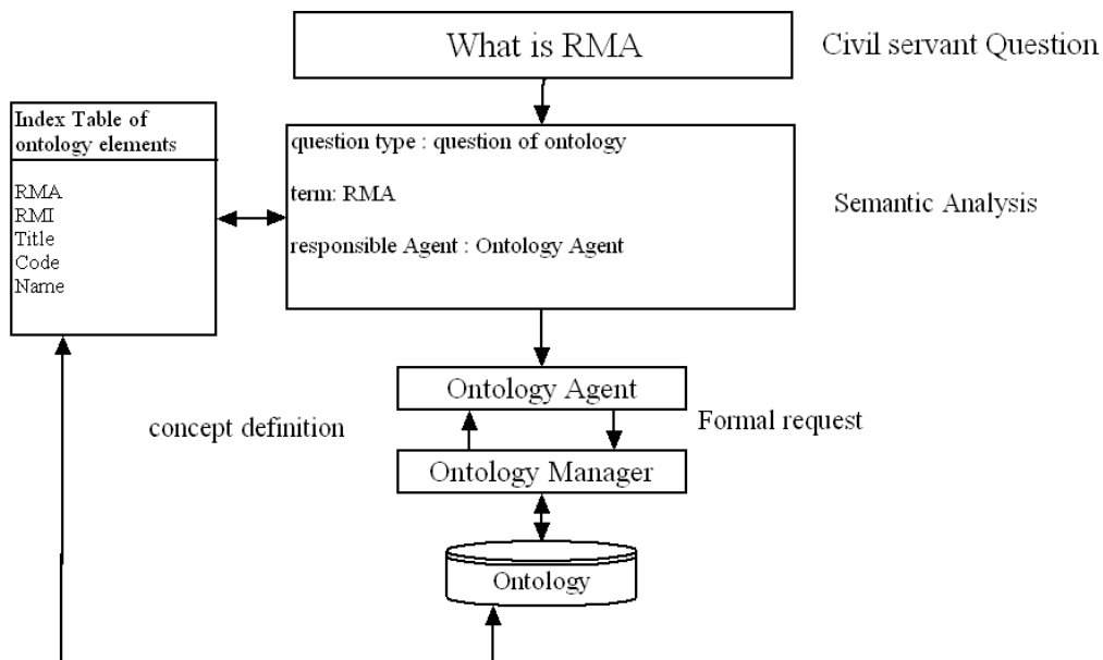
Figure 7: Using index to search a term
