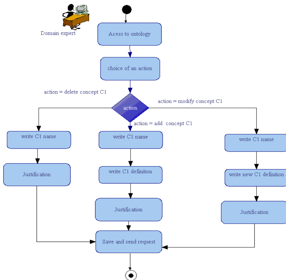
Figure 6: Request for change: actions concerning a concept
